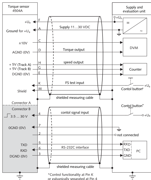
Fig. 1: Pin allocation of the built-in connector A and B (standard)
